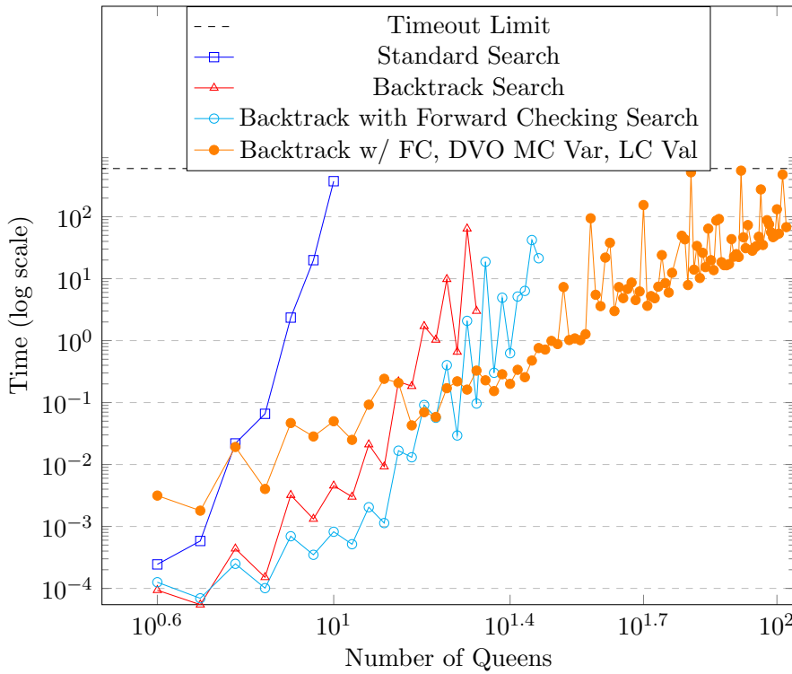
Figure 2: Time in Log vs Num of Queen in Log
