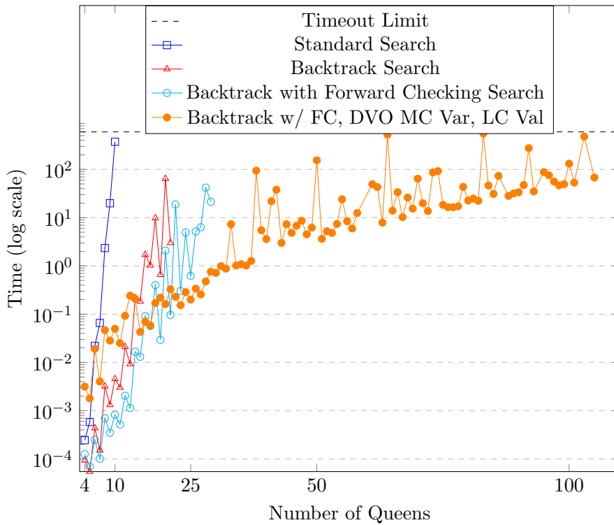
Figure 1: Time in Log vs Num of Queen
